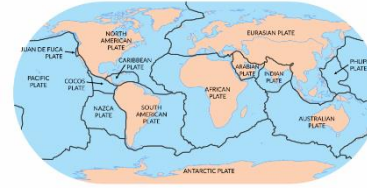
Tectonic plates across the world
