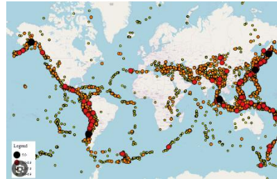
Locations of Earthquakes
